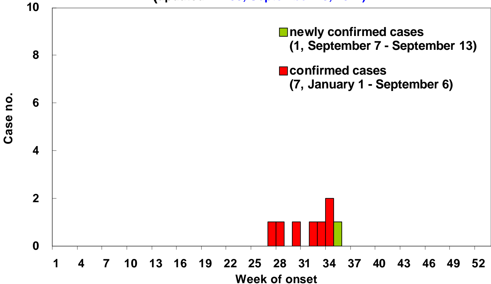
Fig. 2 Trend of EV Infection with Severe Complications, Taiwan, 2011 (updated: 12:00, September 13, 2011)
