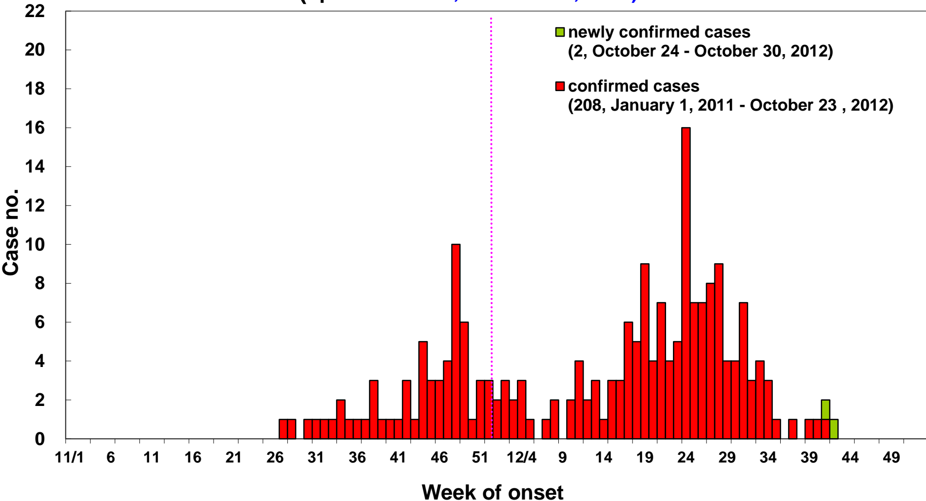
Fig. 2 Trend of EV Infection with Severe Complications, Taiwan, 2011~2012 (updated: 12:00, October 30, 2012)
