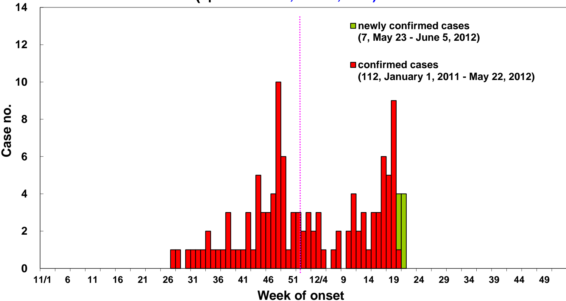
Fig. 2 Trend of EV Infection with Severe Complications, Taiwan, 2011~2012 (updated: 12:00, June 5, 2012)
