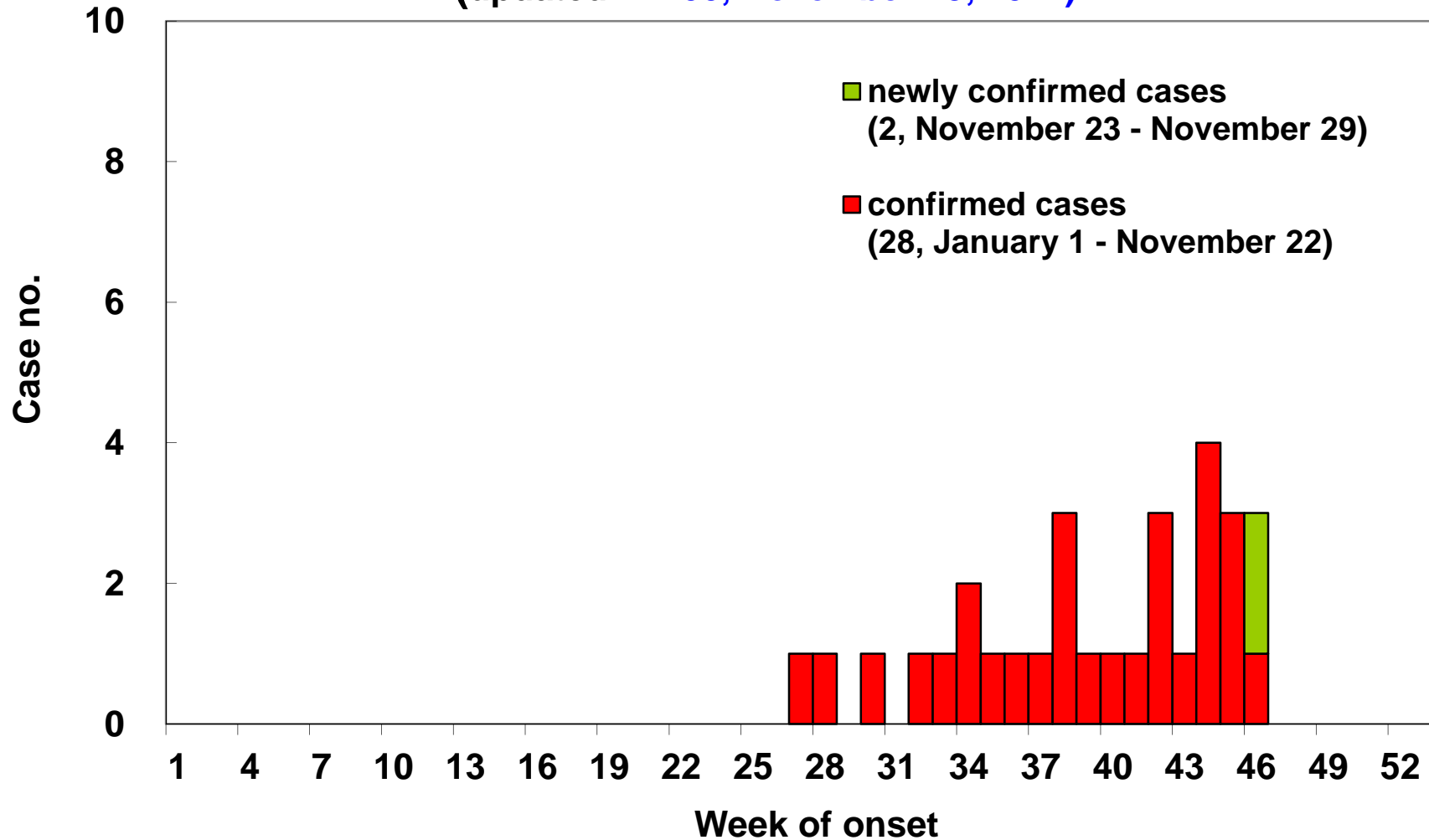
Fig. 2 Trend of EV Infection with Severe Complications, Taiwan, 2011 (updated: 12:00, November 29, 2011)
