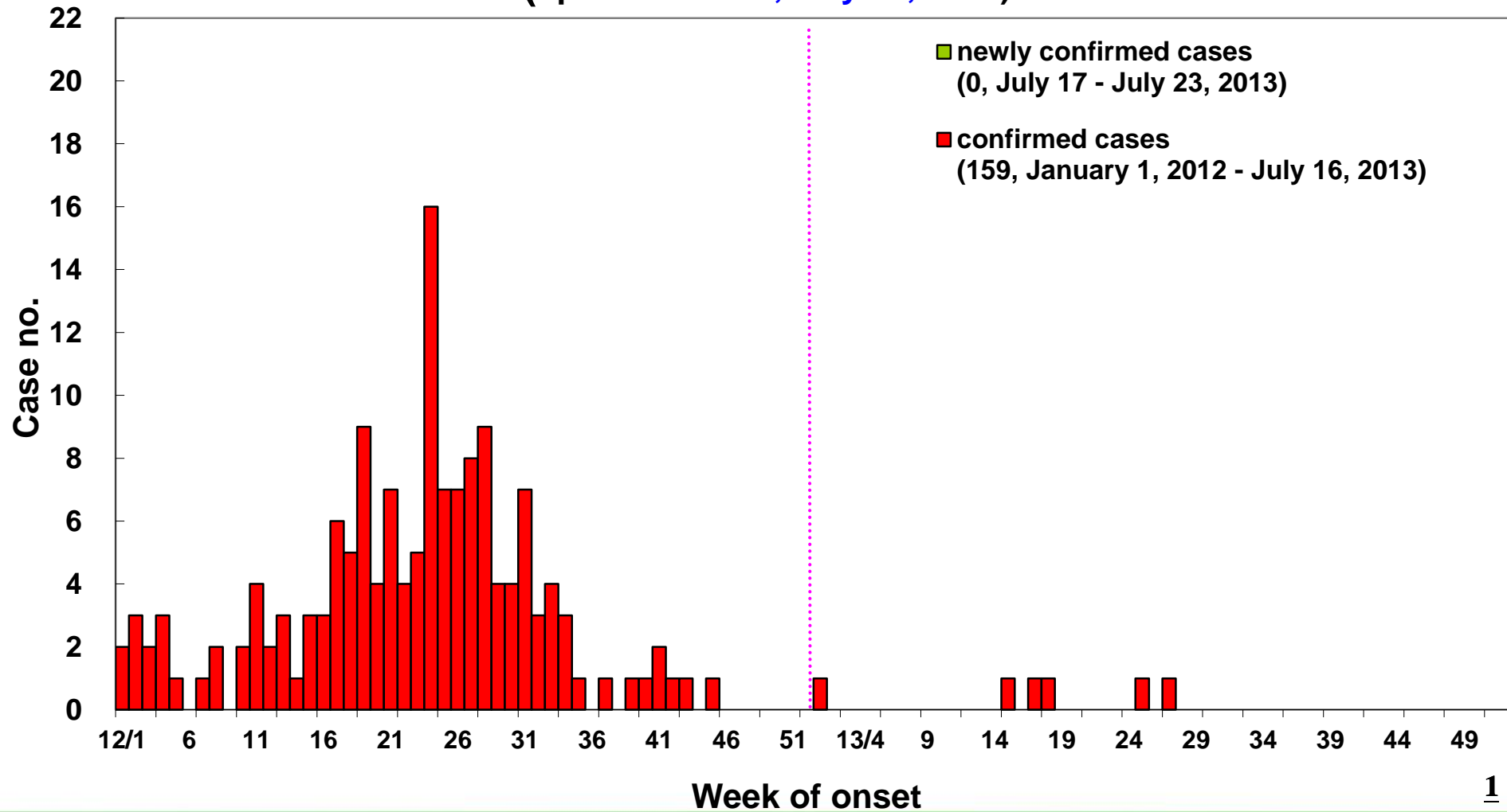
Fig. 2 Trend of EV Infection with Severe Complications , Taiwan, 2012~2013 (updated: 12:00, July 23, 2013)
