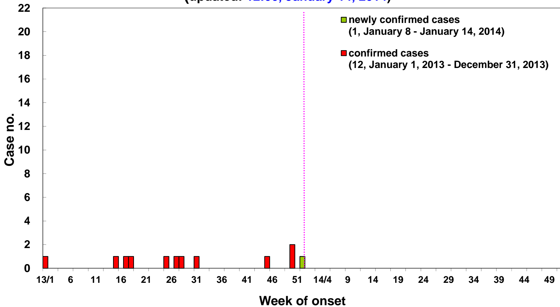
Fig. 2 Trend of EV Infection with Severe Complications, Taiwan, 2013~2014 (updated: 12:00, January 14, 2014)
