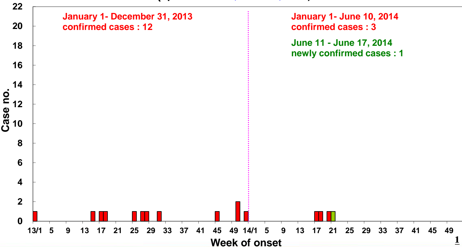
Fig. 2 Trend of EV Infection with Severe Complications, Taiwan, 2013~2014 (updated: 12:00, June 17, 2014)
