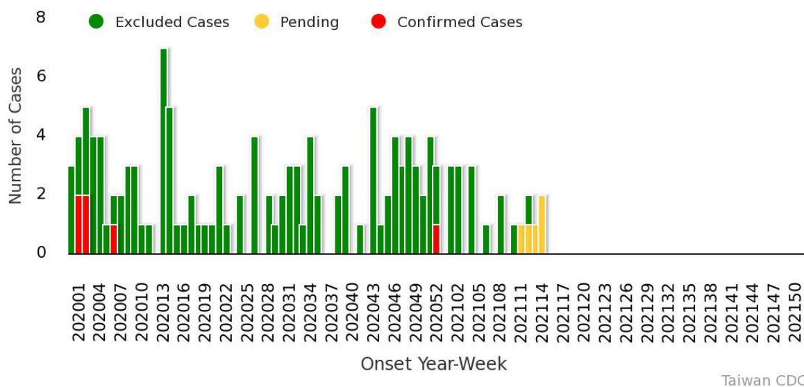
Figure 3. Trend of EVSC, 2020-2021
